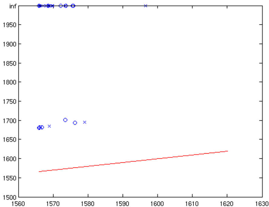
Figure 42: The same picture as Figure 39, but now the corner search adapted to the new boxes of the first probability distribution assumption. Surprisingly many OOU choices (crosses) are now infeasible.
