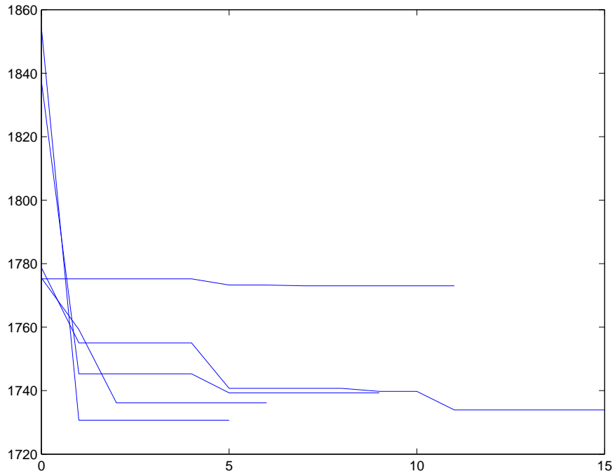
Figure 38: Convergence in 5 different SNOBFIT searches.
