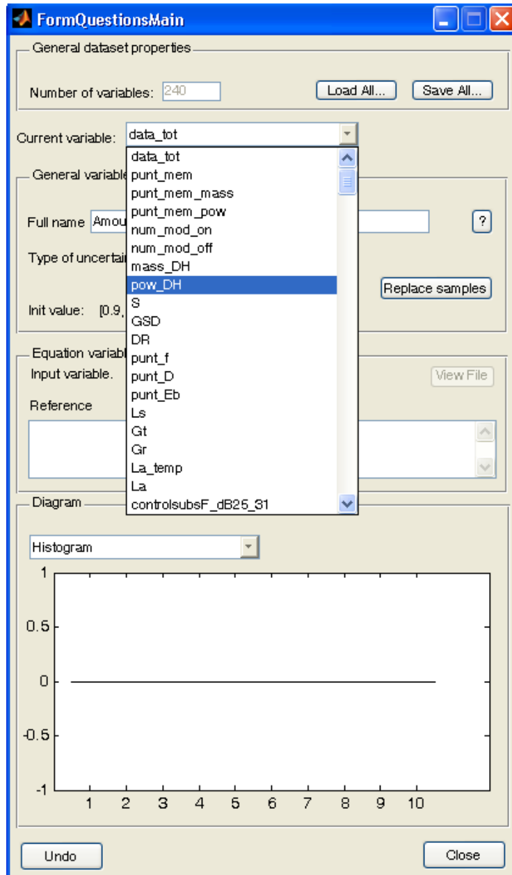
Figure 15: Variable selection.
